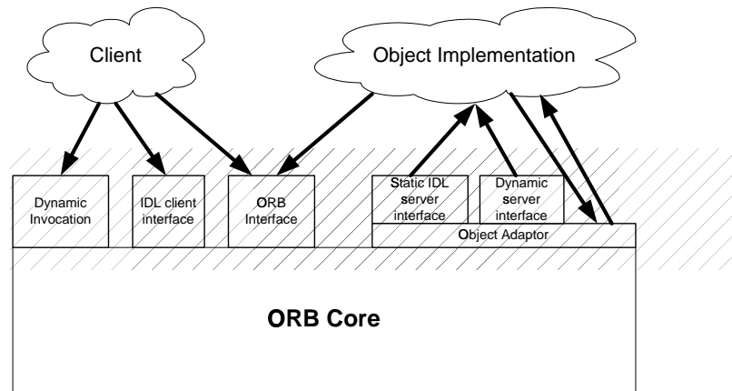
Figure 3-2: The structure of Object Request Broker interfaces
