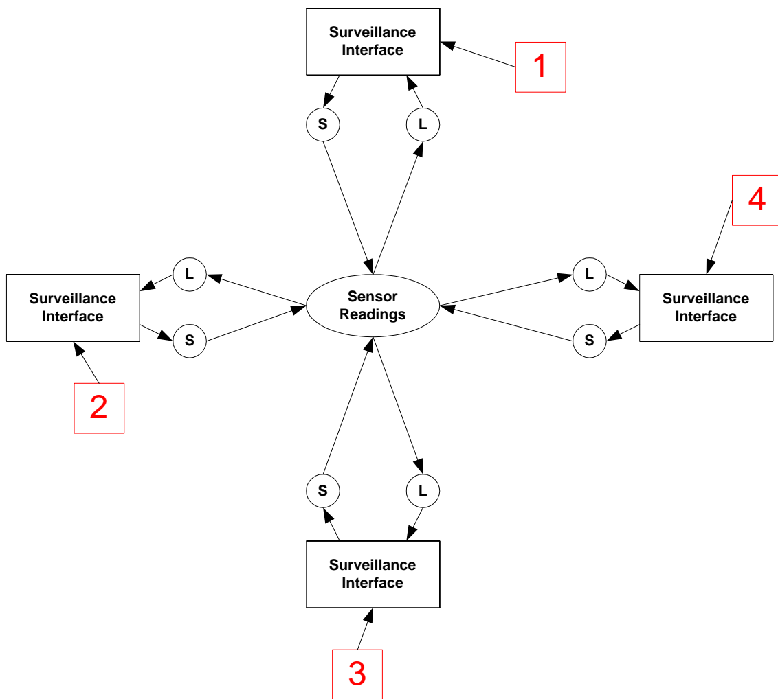
Figure 4-6: Multiregional simulation
