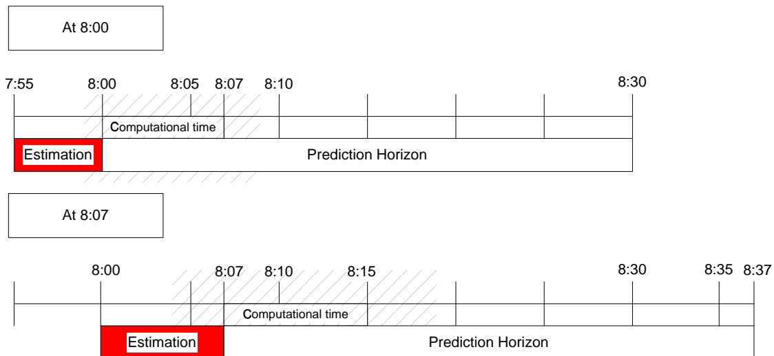
Figure 5-4: DynaMIT: Illustration of the rolling horizon
